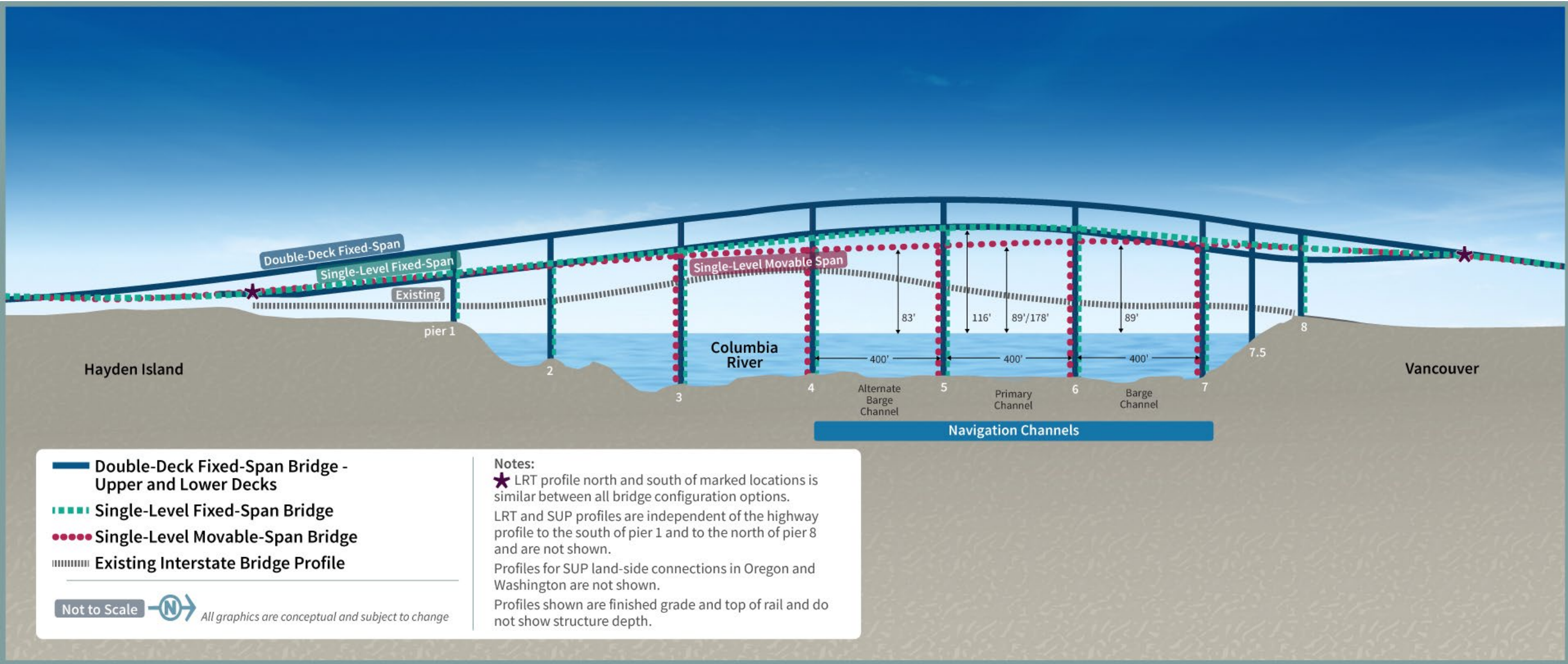
Figure 3-18. Bridge Design Option Profile Comparison
