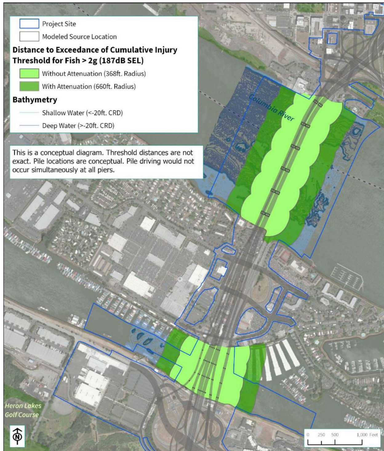
Figure 8-3. Distance to 187 dB SEL Cumulative Injury Threshold for Fish >2 g during Impact Pile Driving – 36 to 48-inch Pile, Single Pile Driver
