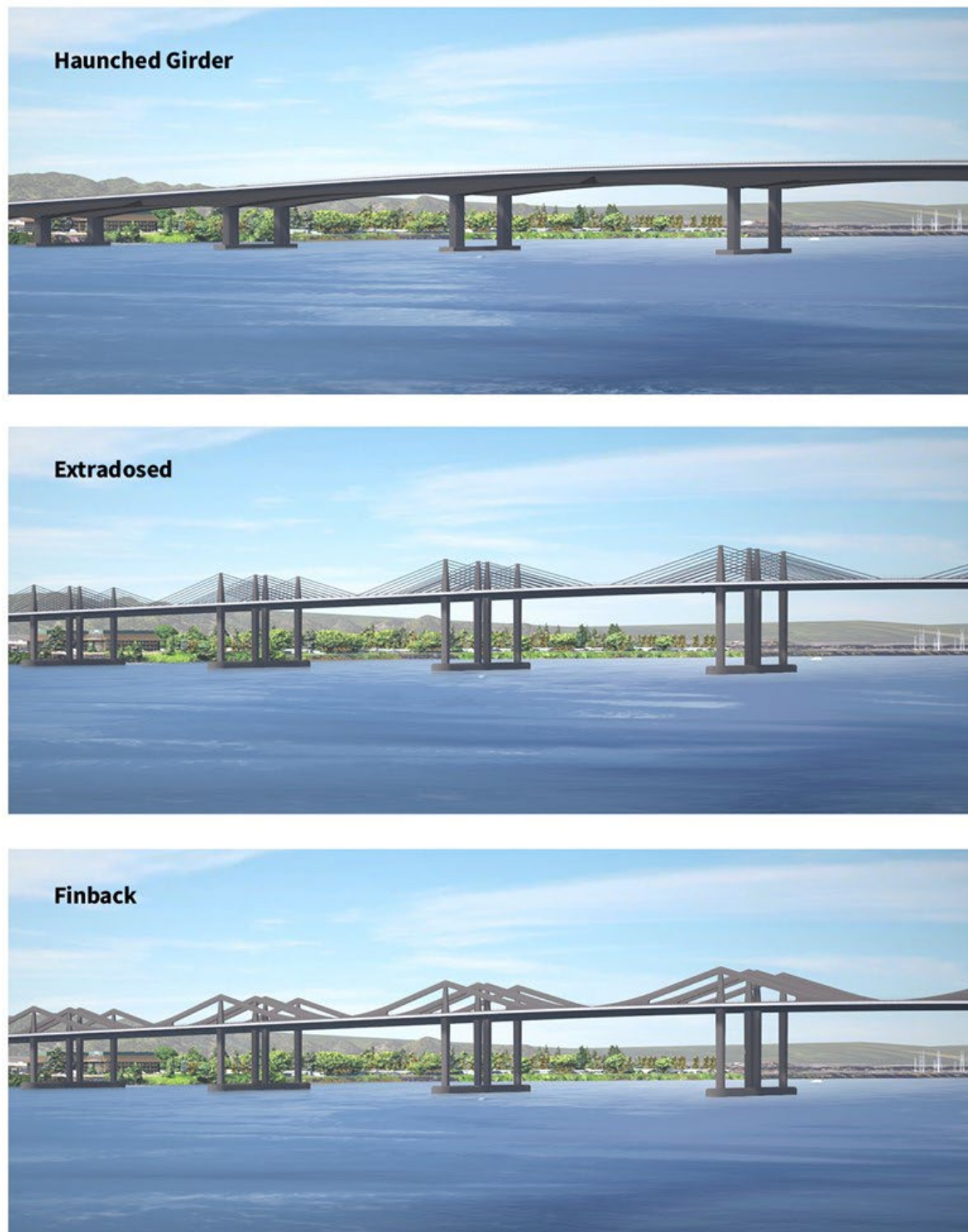
Figure 3-13. Examples of Single-Level Fixed-Span Bridge Types
