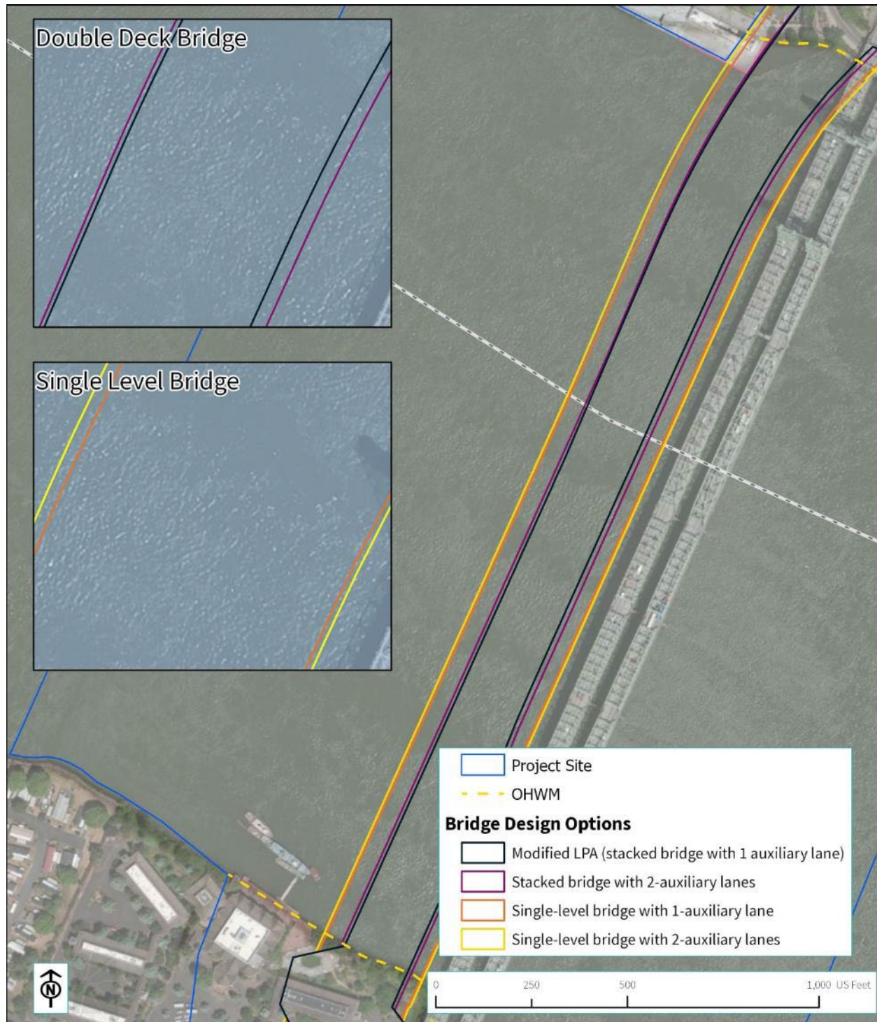
Figure 3-28. Columbia River Bridges – Design Option Bridge Deck Configurations
