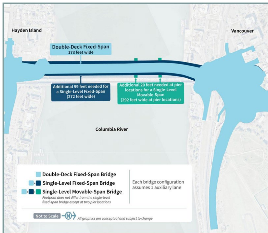
Figure 3-17. Bridge Configurations Footprint Comparison
