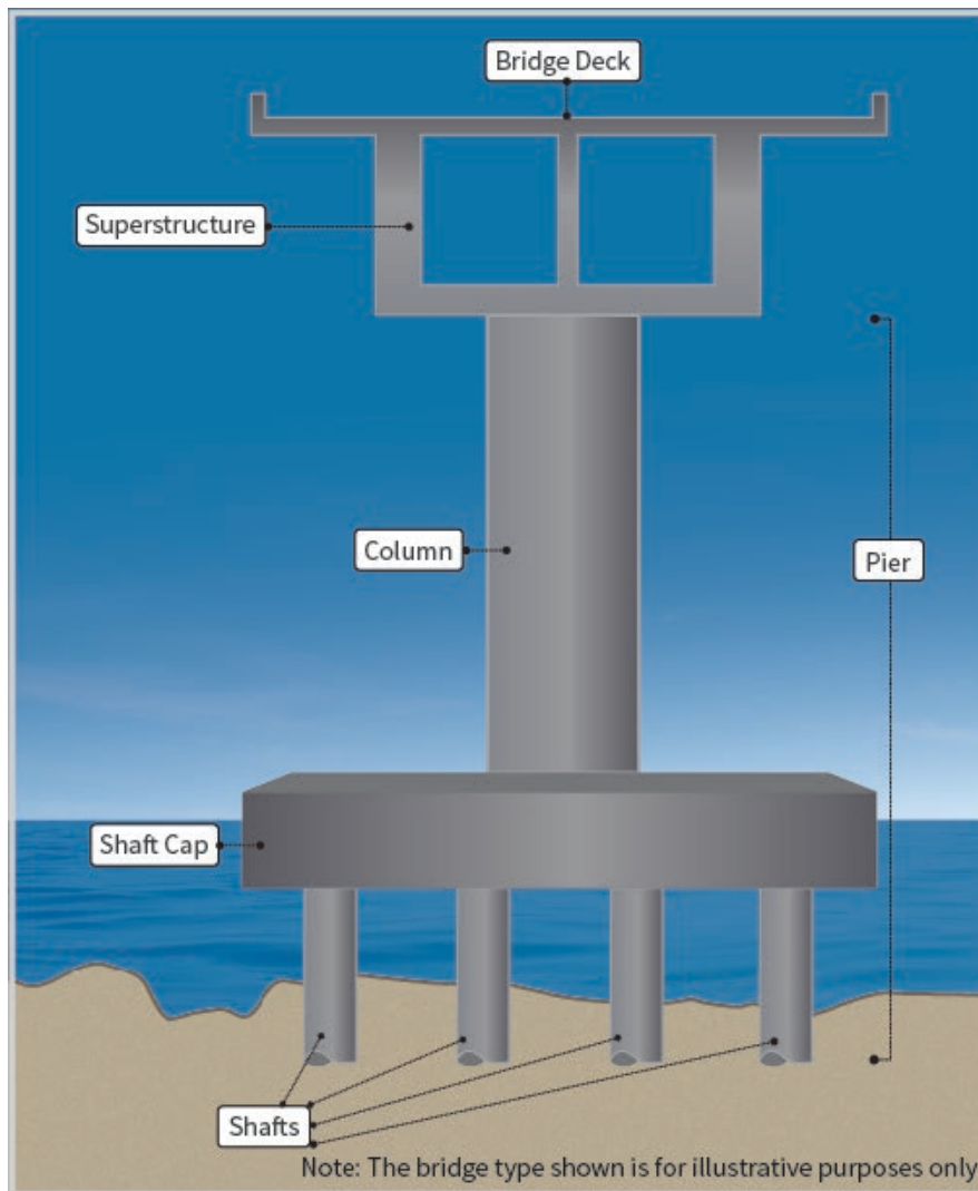
Figure 3-9. Columbia River Bridge Piers – Typical Section
